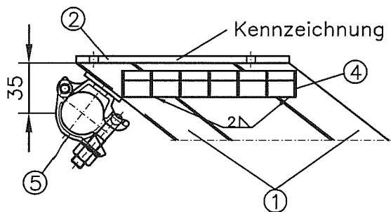
Detail X
