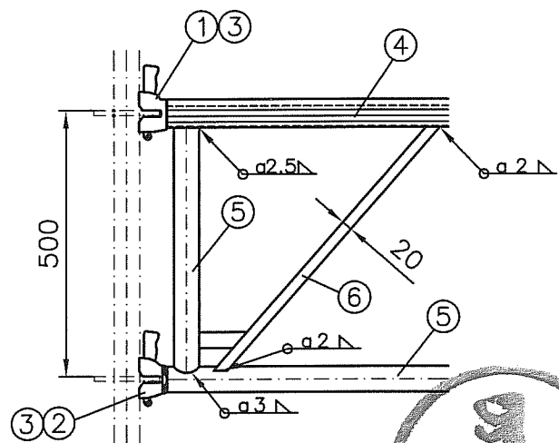
Detail W
