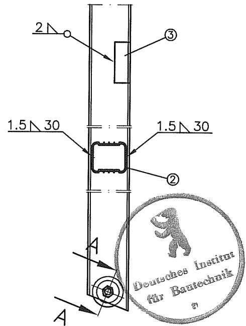
Detail Z
