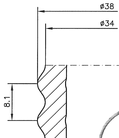
Detail X
